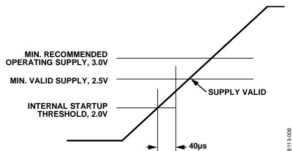
Figure 8. Start-Up Condition, Supply Slew Rate < 12.5 V/ms
